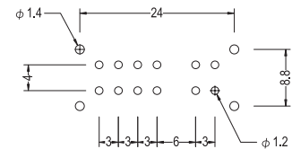
P.C.B. HOLE DETAIL
