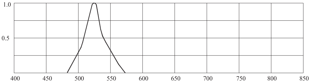
Typical Electrical / Optical Characteristics Curves (25°C Ambient Temperature Unless Otherwise Noted)
