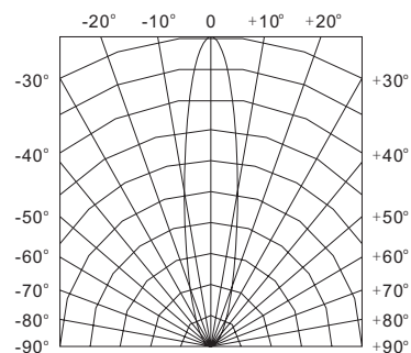
Emitted Angle20° Fig.6 Spatial Distribution
