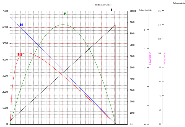
Performance Curve : B3717S-S01
