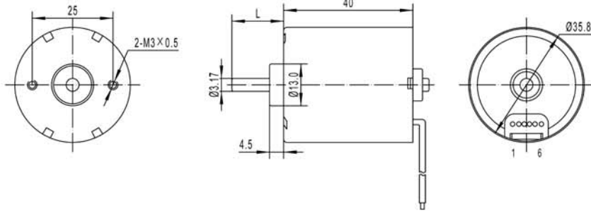
Motor Dimensions (mm)
