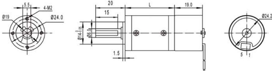
Gear Motor Dimensions (mm)
