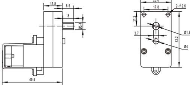
Gear Motor Dimensions (mm)
