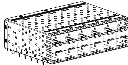
SFP-026 WITHOUT LIGHT PIPES
