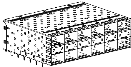
SFP-026L-2A WITH OUTER LIGHT PIPES
