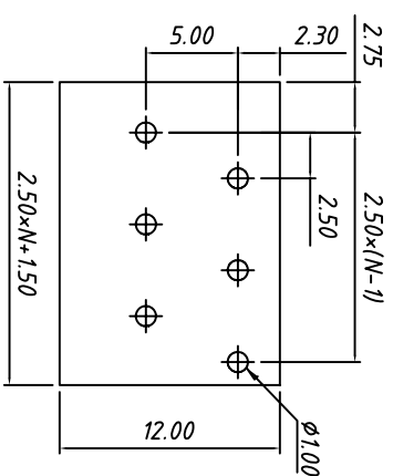
B type PCB LAYOUT
