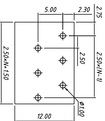
A type PCB LAYOUT
