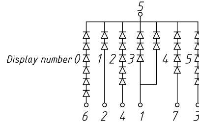
Common Cathode L-KLS9-D-5015 Ax
