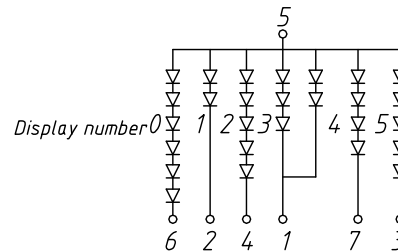
Common Anode L-KLS9-D-5015 Bx
