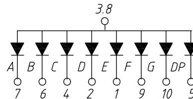
Common Anode L-KLS9-D-8014 Bx
