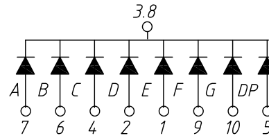
Common Cathode L-KLS9-D-8017 Ax
