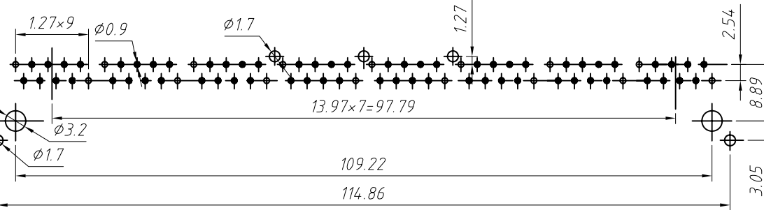
PCB Layout
