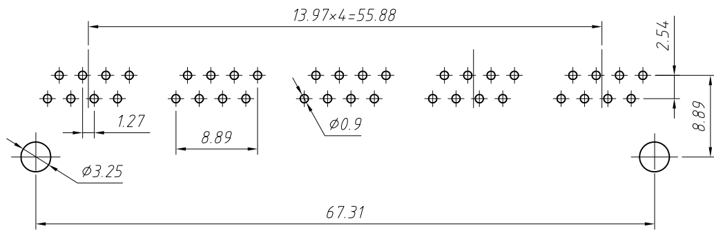
PCB Layout
