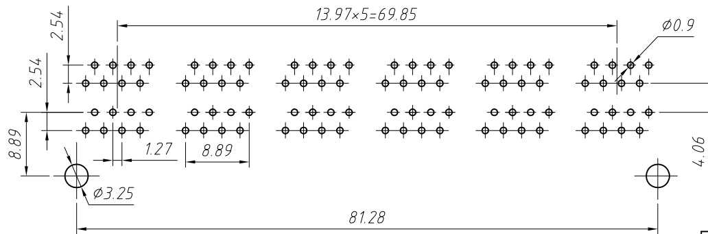
PCB Layout
