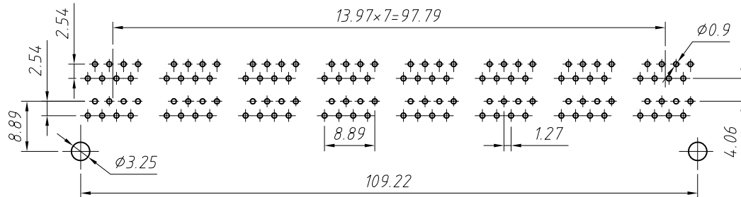
PCB Layout
