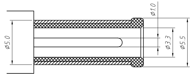
RECOMMENDED PLUG
