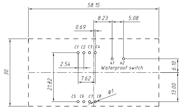
Mounting Hole Dimensions
